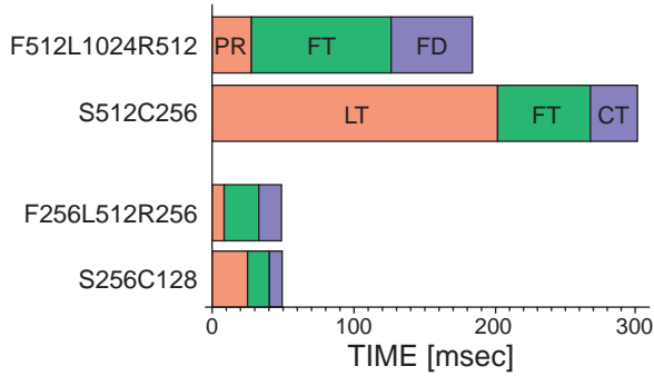
Fig. 3 Comparison of the one time-step computation time between the STM and FTM methods. S... denotes the degree of the spherical harmonic expansion, C... denotes the degree of the Chebyshev polynomial, F... denotes the order of the Fourier expansion, and L... and R... indicates the numbers of grid in latitudinal and radial directions, respectively. Estimated computation times for degrees 256 and 512 are shown.
