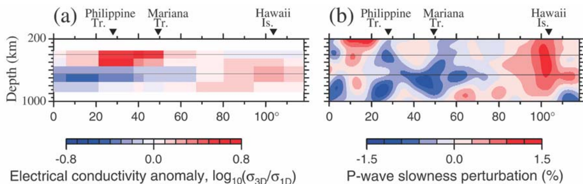
Fig. 4 Profiles of the mantle structure beneath the line through Philippine, Guam and Hawaii. (a) Electrical conductivity anomaly model obtained by using the Earth Simulator. (b) Seismic P-wave slowness perturbation model by Fukao et al. (2003).
