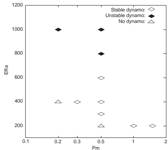
Fig. 1 Diagram of dynamo simulation results. Ordinate represents ERa , and abscissa Pm , where E , Ra and Pm are the Ekman number, the Rayleigh number and the magnetic Prandtl number, respectively. Open diamond represents stable dipolar dynamo, and filled diamond reversing dipolar dynamo, and triangle no dynamo.
