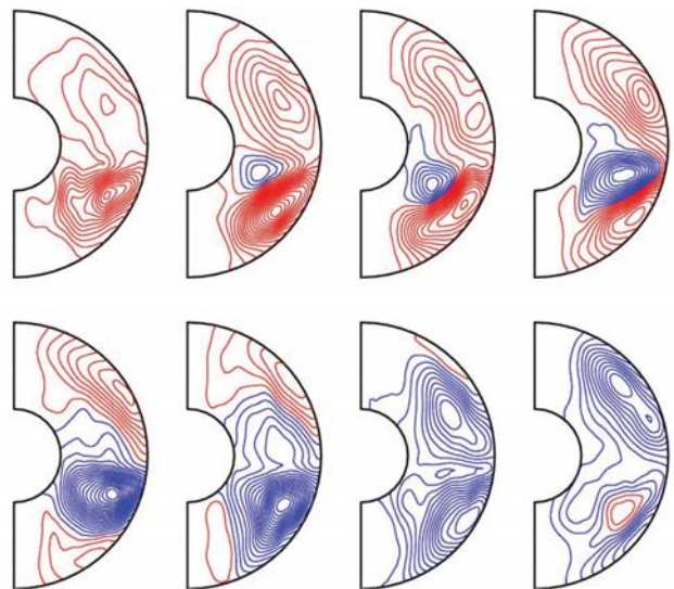
Fig. 2 Time sequence of the dipole field reversal from left to right in top low, then bottom left. Magnetic lines of force are drawn. Parameter values are Ek = 10^{-5} , Ra = 8 \times 10^7 and Pm = 0.5 . Red (blue) lines represent counter-clockwise (clockwise) fields.
