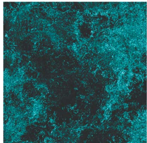
Fig. 4 Intense vorticity regions obtained by the 2048 3 DNS.
