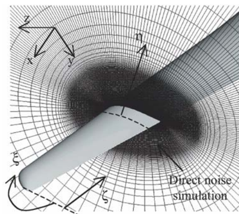
Fig. 6 Computational grid of airfoil section
