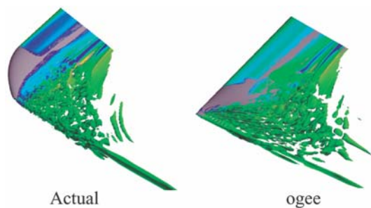
Fig. 7 Vorticity \omega_x Isosurfaces (Color denotes pressure)
