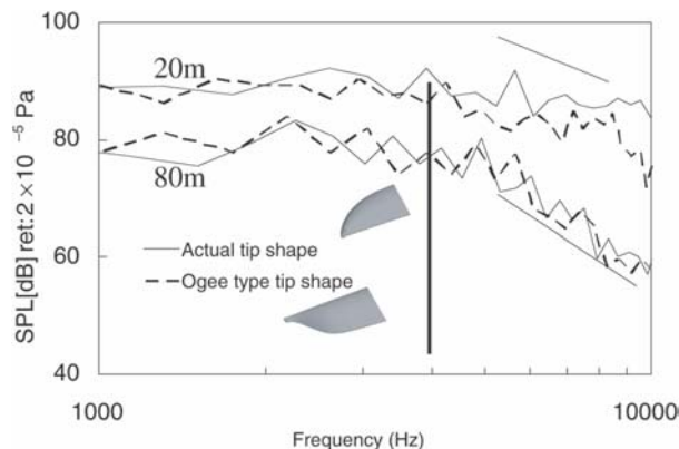
Fig. 9 Sound pressure level at two locations – Simulation results
