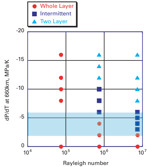
Fig. 2 A regime diagram of convective flow patterns in the plane of |dP/dT_{660}| versus Ra . Ra_H is fixed to be 1.4 \times 10^8 . The shaded region indicates the range of dP/dT_{660} of the Earth estimated from the high-pressure experimental results.
