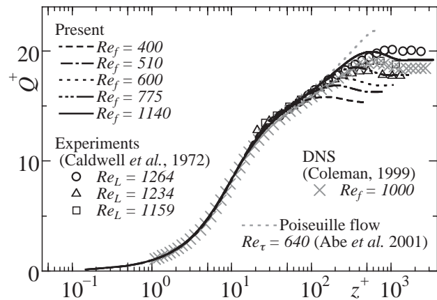
Fig. 2 Mean velocity profiles.
