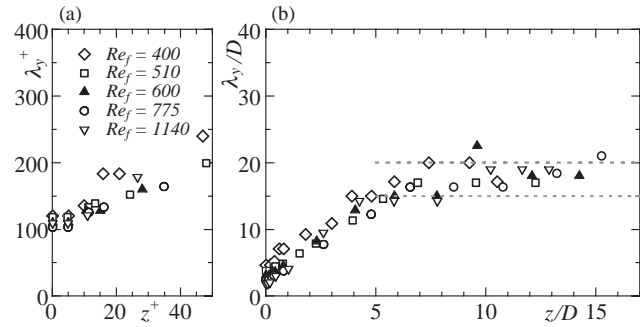
Fig. 19 Spanwise wavelength of the maxima of the pre-multiplied spectra normalized by (a) the wall-unit and (b) the viscous Ekman depth D .
