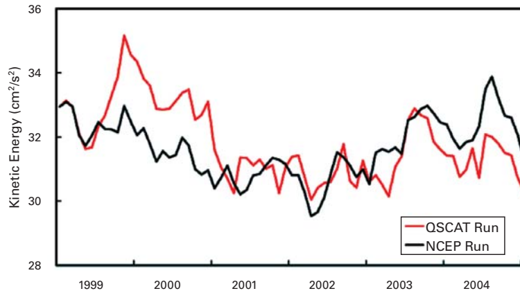
Fig. 2 Time series of global (75°S–75°N) mean kinetic energy ( \text{cm}^2 \text{s}^{-2} ) from 1999 to 2004 based on the (red curve) QSCAT and (black curve) NCEP runs.
