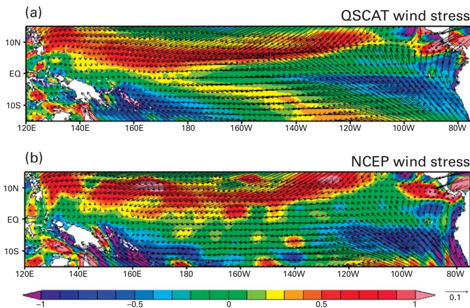
Fig. 6 Distributions of mean wind stress curl in common logarithm scale (color, unit: 10 -7 N m -3 ) and vectors (N m -2 ) averaged from 2001 to 2004 in the equatorial Pacific in (a) the QSCAT satellite observation and (b) the NCEP/NCAR reanalysis.
