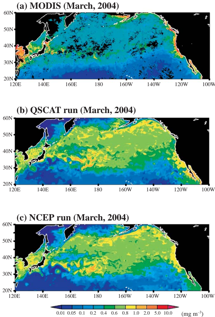
Fig. 10 Distribution of surface chlorophyll concentration (mg m -3 ) in March: (a) MODIS satellite image, (b) QSCAT run, and (c) NCEP run.
