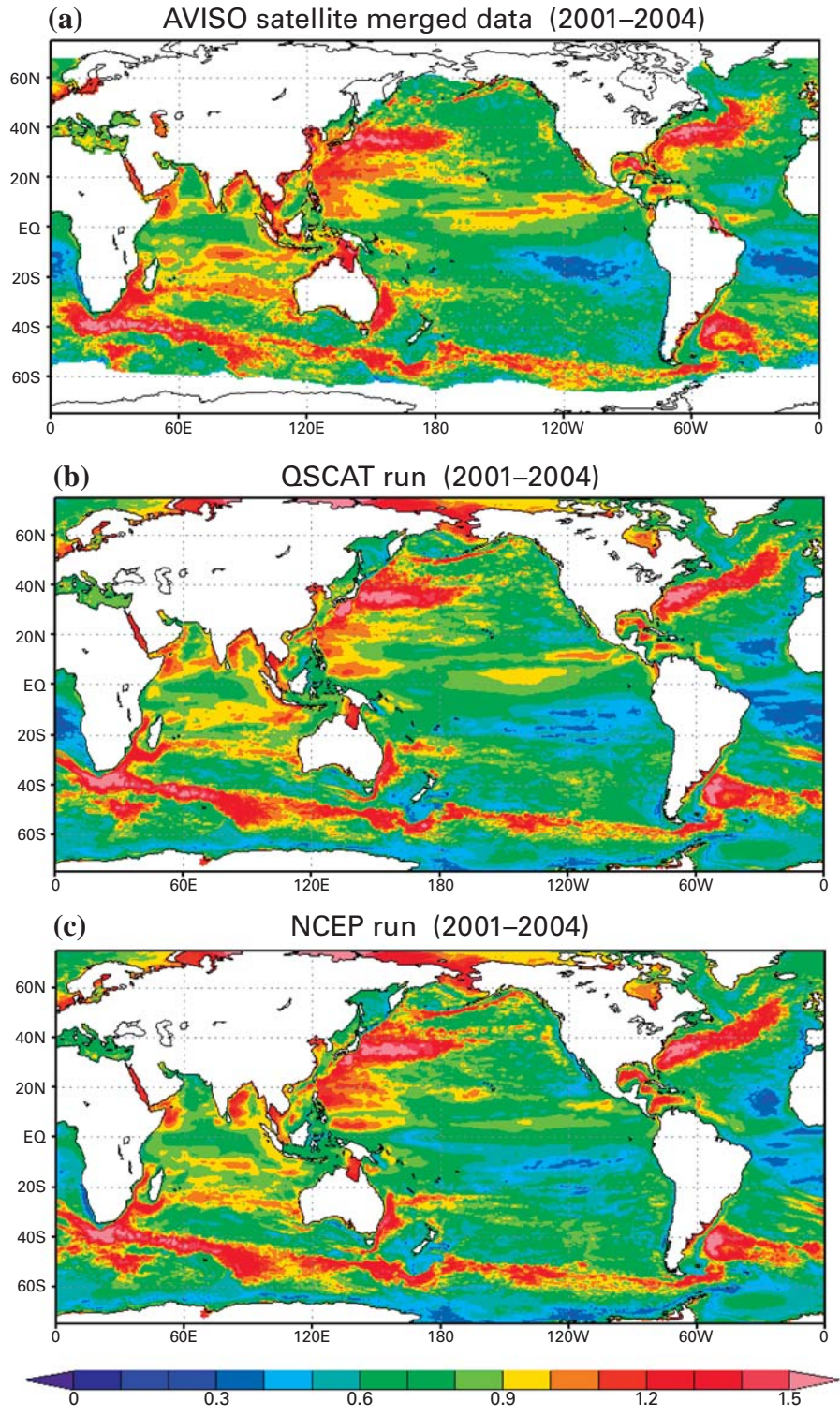
Fig. 4 Distributions of root-mean-square variances of sea surface height anomalies in common logarithm scale (cm) for 2001–2004 based on (a) the AVISO satellite observation and the (b) QSCAT and (c) NCEP runs.
