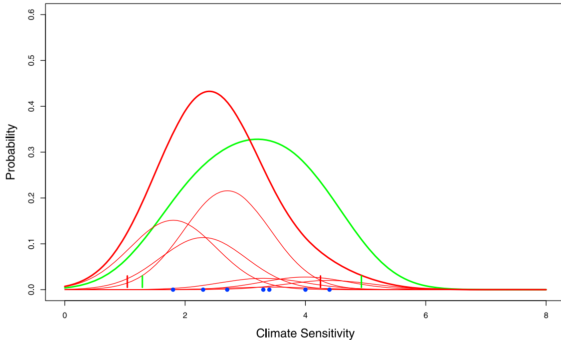
Figure 3. Bayesian approach to estimating climate sensitivity. Green curve shows prior, thick red curve is posterior and vertical bars show 5–95% range. Blue dots show model values and thin red curves indicate weighted contribution of each model to the posterior.
