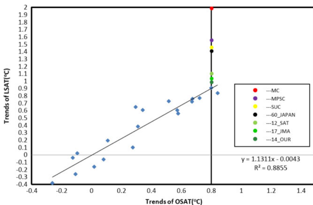
Figure 2. The blue diamonds are the centennial linear temperature trends over land and ocean for the Japan region, from the simulations of 19 CMIP3 models. The vertical line crossing the x -axis at 0.8^{\circ}\text{C} illustrates the observed trend of COBE-SST and cuts the trend line through the CMIP3 results at 0.90^{\circ}\text{C} . The y -axis values for the coloured dots along this vertical line are the observed trends from the terrestrial Japanese station data. The red dot is the average trend of the 9 megacities, the purple dot is the average of the 46 mega plus suburban cities, yellow dot is the average trend of 37 suburban cities, the green dots are the average trends for the various sets of rural stations and the black dot is the average for all the 60 stations.
