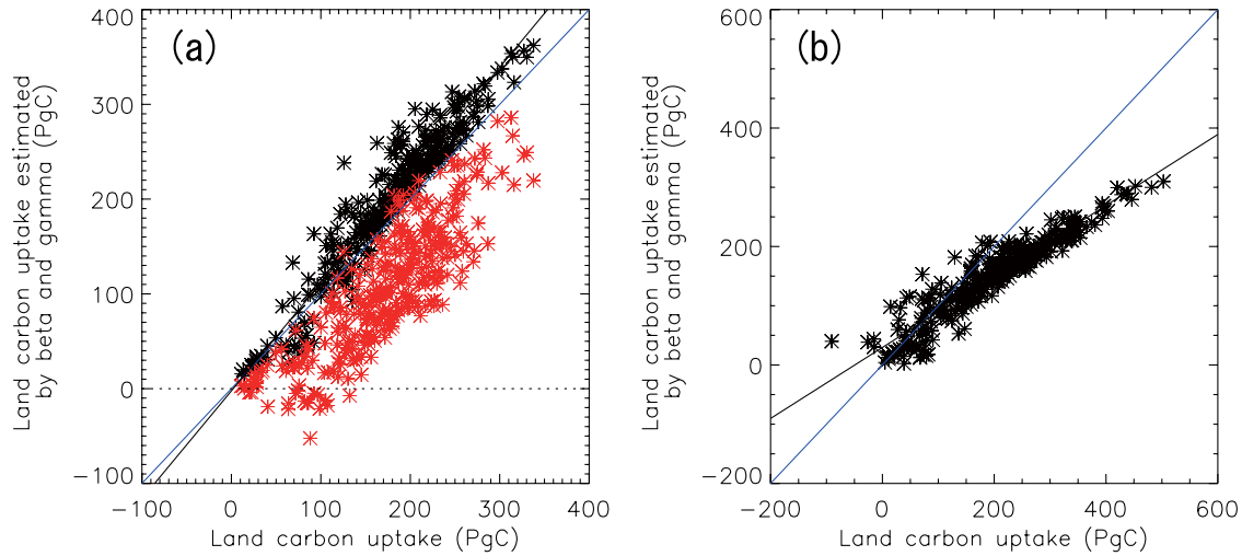
Fig. 5. Non-constancy in \beta_L and \gamma_L presented as the estimated C_{uL} . (a) Modelled and estimated C_{uL} by \beta_L C + \gamma_L T up to 66th year for 1% p.a. scenario ( C , T are change in atmospheric \text{CO}_2 concentration and in temperature from the first year). Black: estimation using \beta_L and \gamma_L up to 66th year, red: estimation using \beta_L and \gamma_L up to 116th year. Black and blue lines are regression line for black marks and y = x . (b) Modelled and estimated C_{uL} from 1850 to 2100 for RCP4.5 scenario. Estimation is using \beta_{L66} and \gamma_{L66} in 1% p.a. scenario. Black and blue lines are regression line and y = x .
