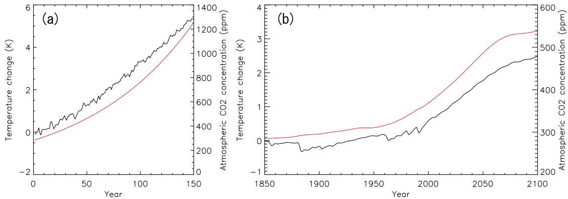
Fig. 1. Atmospheric CO 2 concentration and global mean surface air temperature for the two experiments. (a) The 1% p.a. scenario, (b) RCP4.5 scenario. For both of (a) and (b), black lines are temperature rise (using left axis) and red lines show the atmospheric CO 2 concentration (using right axis).
