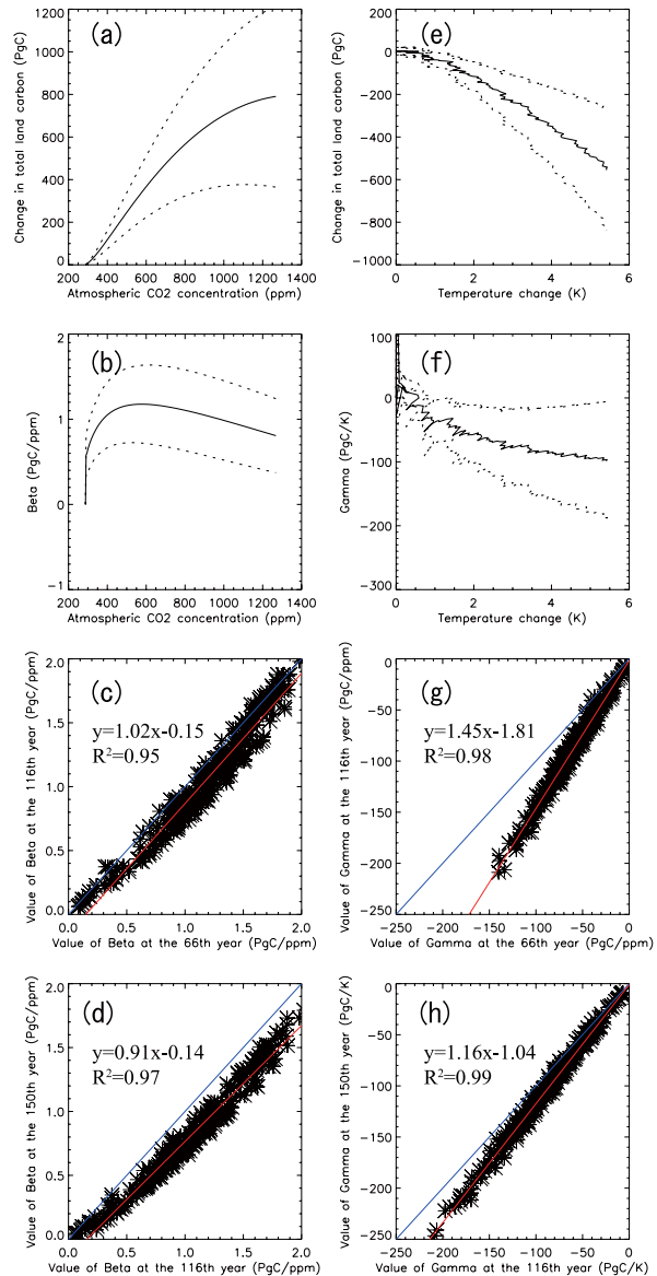
Fig. 3. Nonlinearity of land carbon sensitivities in the 1% p.a. experiment. (a) Change in land carbon for increasing \text{CO}_2 concentration in the BGC coupled run, (b) change in \beta_L , (c) Relationship between \beta_L s calculated at the 66th and at the 116th years. (d) relationship between \beta_L s calculated at the 116th and at the 150th years. The blue and red lines in (c) and (d) are y = x , and the regression line (the coefficients of the line and the coefficients of determination is also presented). (e) Change in land carbon for increasing air temperature in the radiatively coupled run, (f)–(h) are same as (b)–(d) but for \gamma_L .
