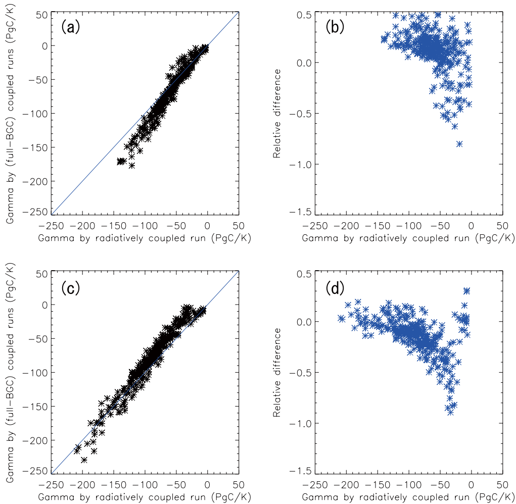
Fig. 4. Relationship between \gamma_L s calculated by radiatively coupled run and by full-BGC coupled runs for 1% p.a. scenario. (a) The values calculated by full-BGC coupled run up to 66th year. The blue lines show y = x . (b) The difference of two methods (presented is (\gamma_{full-BGC} - \gamma_{rad})/\gamma_{rad} ). (c) (d) are same as (a) (b) but for 116th year.
