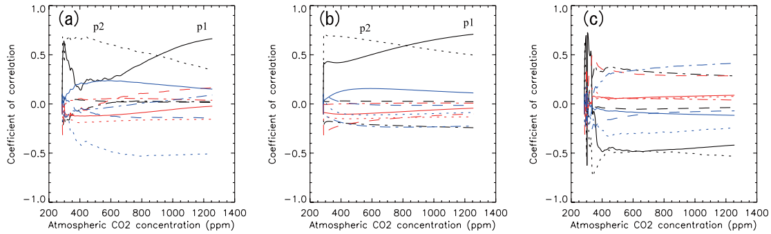
Fig. 6. Change in coefficient of correlation between parameter values and change in total land carbon in the 1% p.a. scenario. (a) To the total land carbon, (b) to \beta_L , (c) to \gamma_L . In all figures, black/red/blue lines are p1–4/p5–8/p9–12, solid/dotted/dashed/dash-dot lines are p1,5,9/p2,6,10/p3,7,11/p4,8,12.
