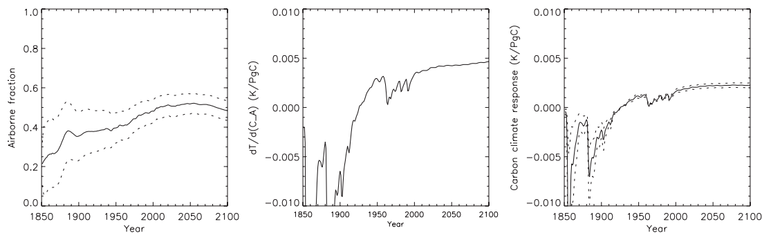
Fig. 2. Carbon Climate Response. (a): Airborne fraction ( A ) (b): dT/dC_A , the ratio of temperature change (K) to change in airborne carbon (PgC), (c): Carbon Climate Response. Average (solid) ± 1 standard deviation (dotted) are presented in (a) and (c).
