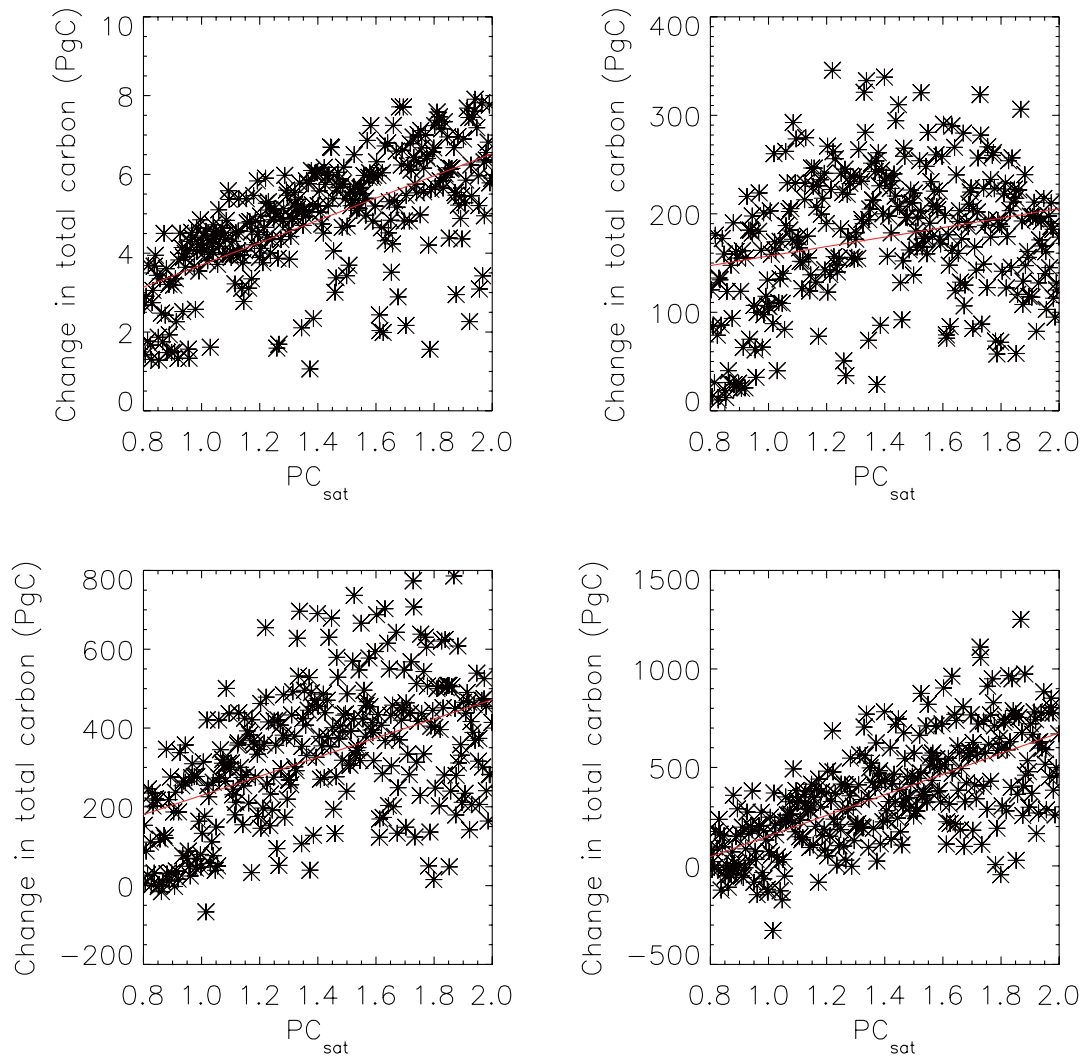
Fig. 7. Relationship between PC_{sat0} and the change in total carbon in the 1% p.a. experiment. (a) At the 5th year (about 300 ppm), (b) at the 66th year (about 550 ppm), (c) at the 116th year (about 900 ppm), (d) at the 150th year (about 1270 ppm). Red lines are linear regression.
