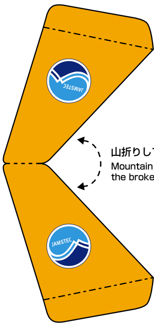
部品C (垂直尾翼) C (Vertical tail fin)
