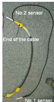
"Sea Snake" Floating Thermistor
