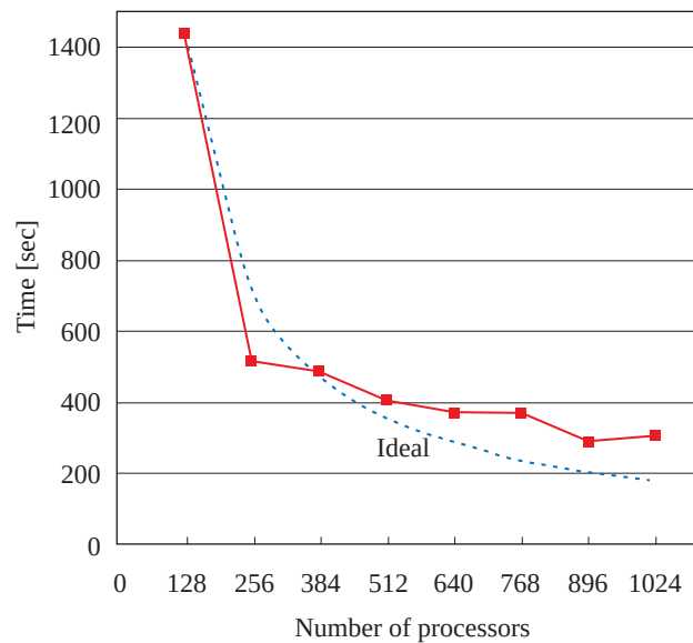
Fig. 14 Scalability in total computation time of elastostatic analysis of the ABWR model on the Earth Simulator
