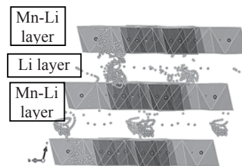
Fig. 3: Motions of Li atoms which existed in Li layer at first.
