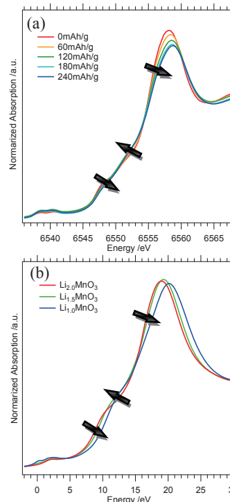
Fig. 1: (a) In-situ XANES and (b) Simulated spectra of Mn K-edge.
