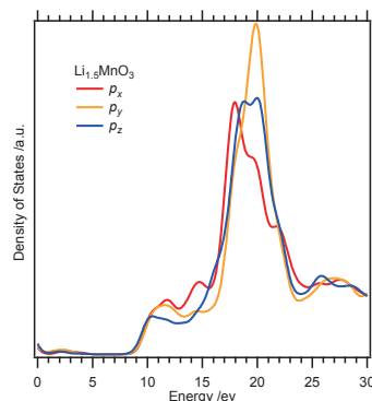
Fig. 2: Simulated 4p PDOS of Mn for \text{Li}_{1.5}\text{MnO}_3
