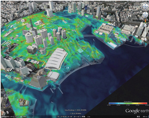
Fig. 2 Air temperature on the surface.
