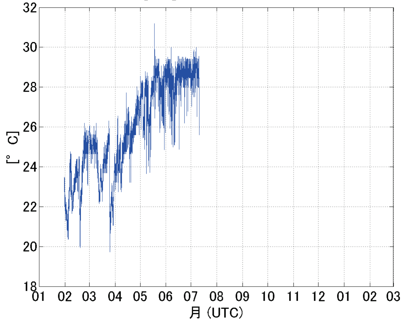
温度[° C] 2012/01/31~13/02/20
