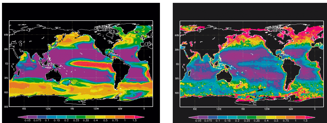
Fig. 1 Annual mean chlorophyll obtained by the model (a) and satellite measurements with CZCS (b). Units are \text{mgChl/m}^3 .
