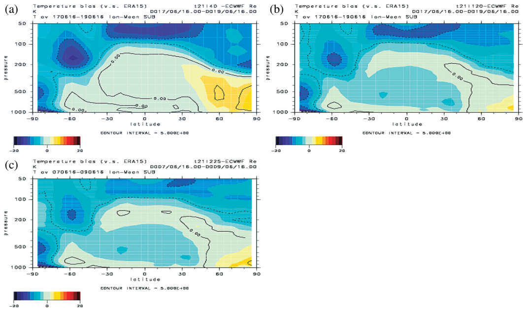
Fig. 3 Zonal mean temperature bias in June for vertical resolution of (a) 1500m, (b) 500m and (c) 200m. Reference temperature is ERA15. The contour interval is 5 K.
