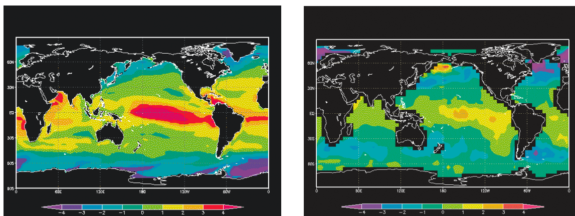
Fig. 2 Annual air-sea exchange of \text{CO}_2 obtained by the model (a) and observations (Takahashi et al., 1999; b). Positive values mean fluxes from the ocean to the atmosphere, and vice versa. Units are \text{molC/m}^2/\text{yr} .
