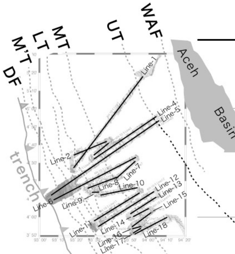
Figure 1 The survey lines (heavy black lines) during the KH10-5 cruise. Main structural features (dashed): WAF, West Andaman Fault; UT, Upper Thrust; MT, Middle Thrust; LT, Lower Thrust; M'T, Main Thrust. DF, Deformation Front. UT and LT, are depicted according to Sibuet et al. (2007); MT according to Hirata et al. (2010).
